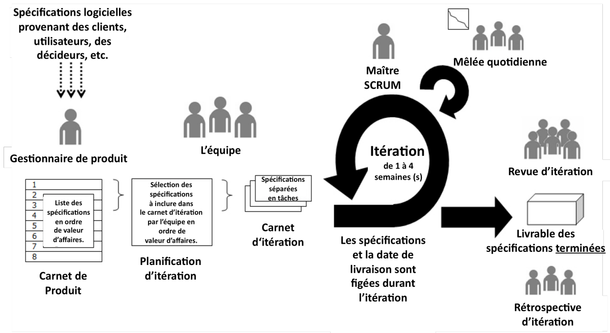
Figure 5 Processus SCRUM [Sutherland 1993]
